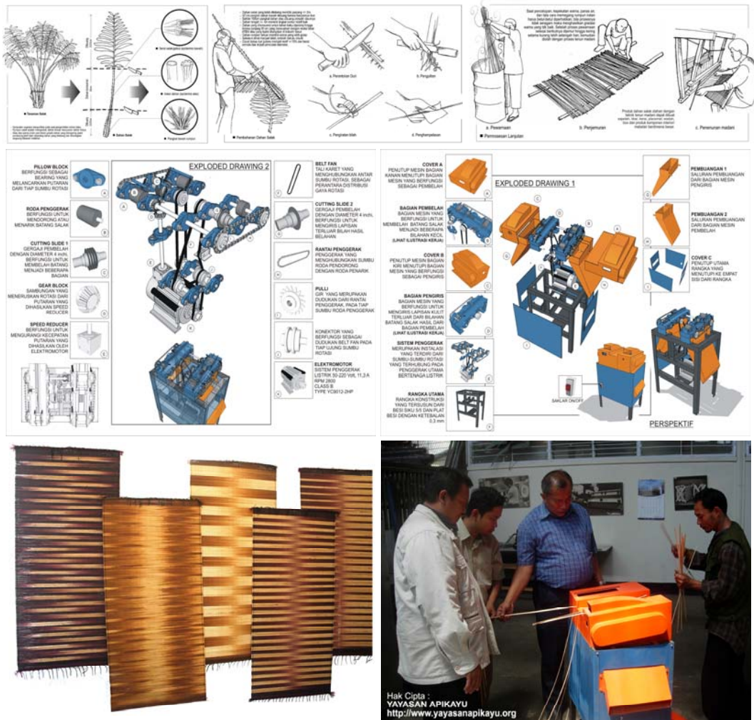
Palm Tree (Salacca) Waste R&D and Stripping Machine Development, 2006 Deny Willy Junaidy, Oemar Handoyo
